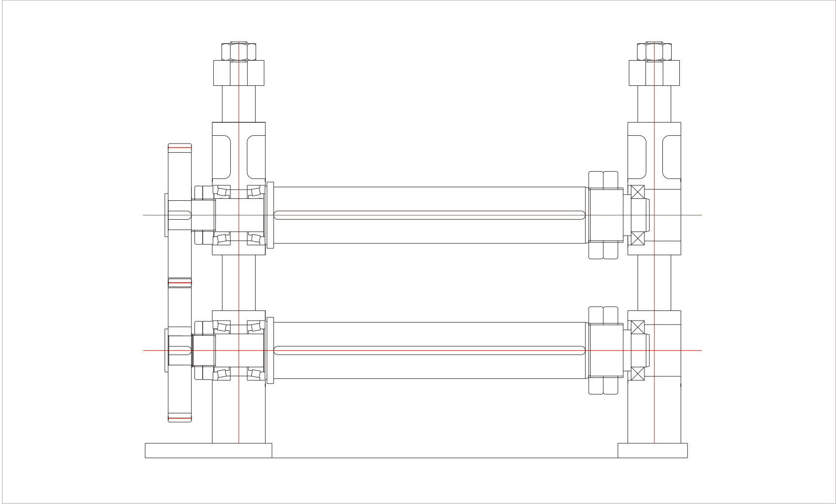
Spur Gear Drive Single Purpose
