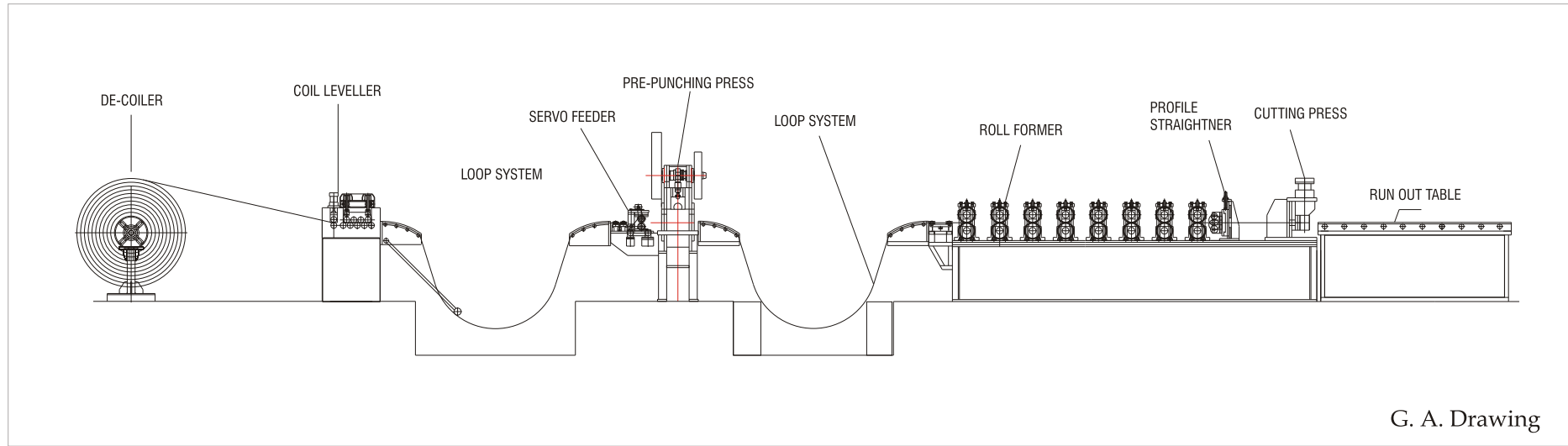
Roll Forming Line
