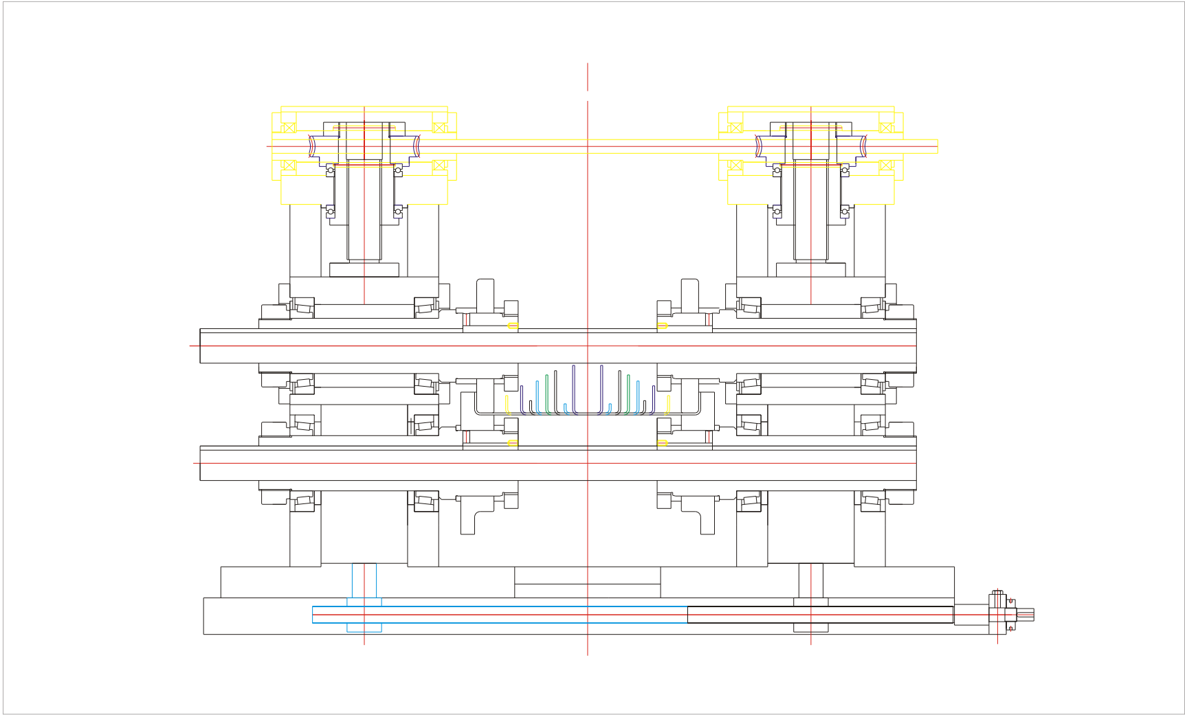
Sliding Type Unit for Inline Profile Dimension Change
